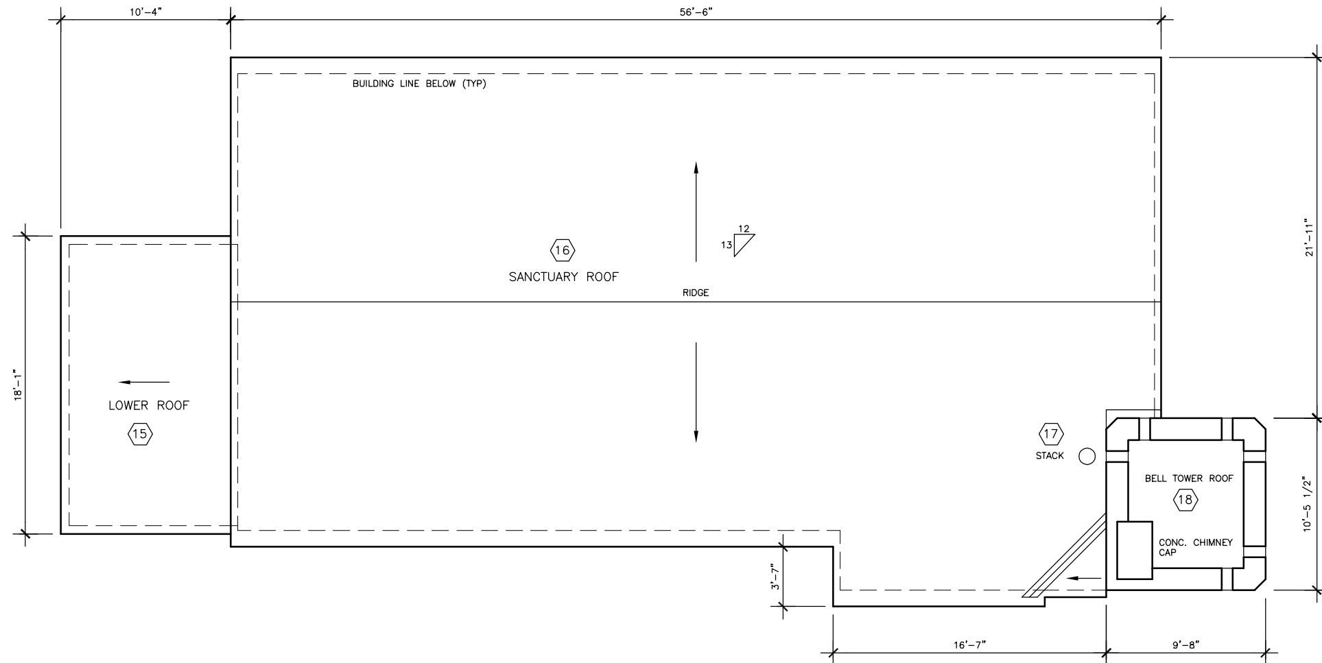
A ROOF PLAN SCALE: 1/4" = 1'-0" D:\CAD\0302
